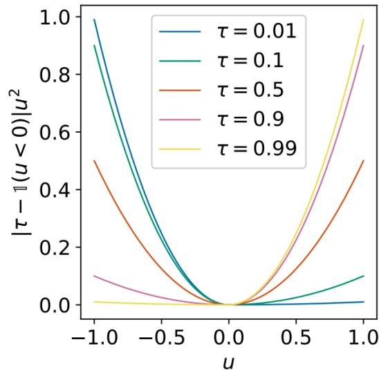
Figure 2: Expectile loss function visualized for different values of \tau .
